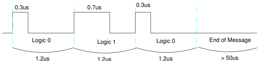
Figure 2: Timing for logic 0 and logic 1 for a NeoPixel
