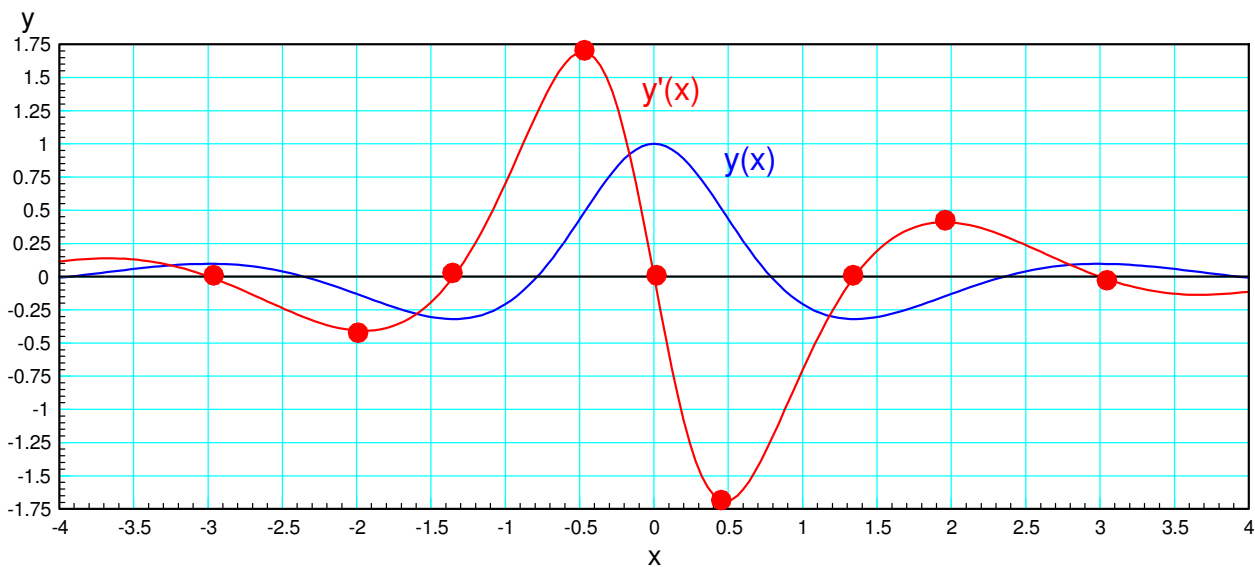
Figure 11: Connect these points to find the derivative of y(x)
