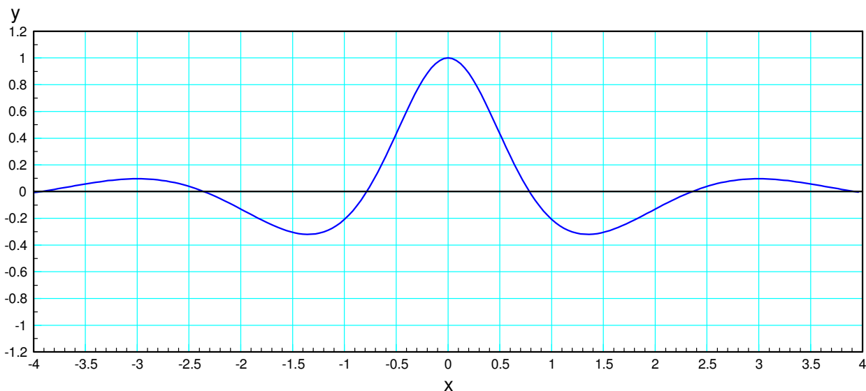
Figure 9: Graph of y = f(x) .
