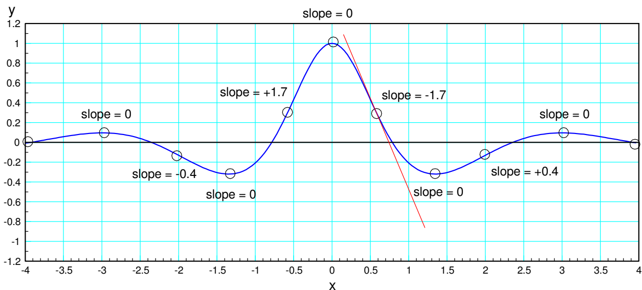
Figure 10: To find the derivative using graphical methods, determine the slope at several points
