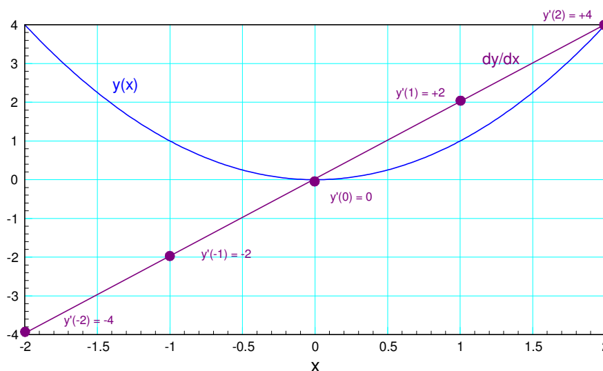
Figure 6: The derivative of y(x) is found by connecting the points
