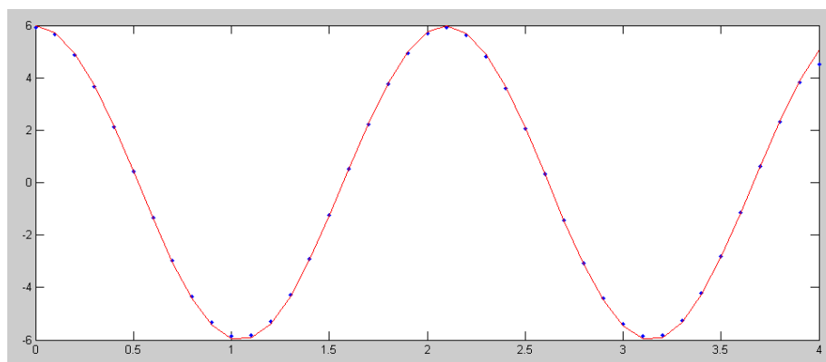
Figure 15: Comparison of the actual derivative of 2\sin(3t) (red) and its computed value (blue dot).
