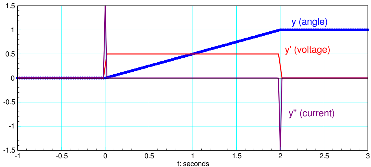
Figure 22: Implied voltage and current required to follow the prescribed path, found using differentiation
