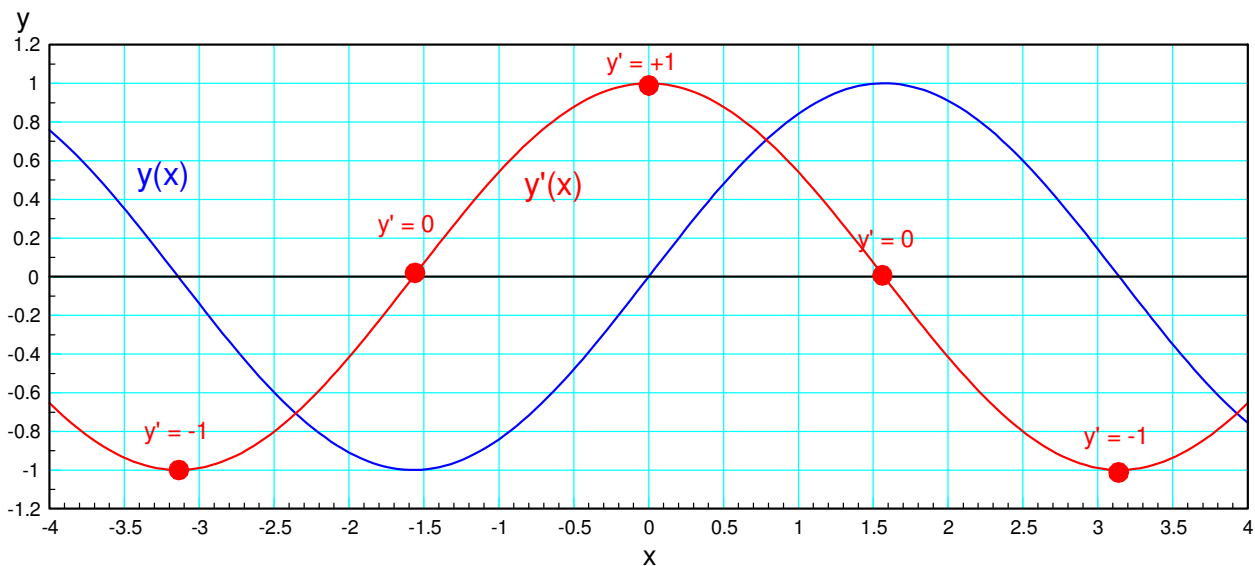
Figure 8: Connect the points to come up with the derivative of y(x)
