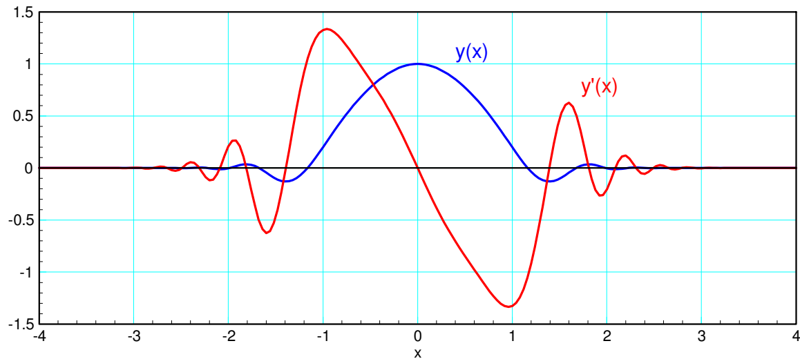
Figure 16: y(x) and its derivative using numerical differentiation
