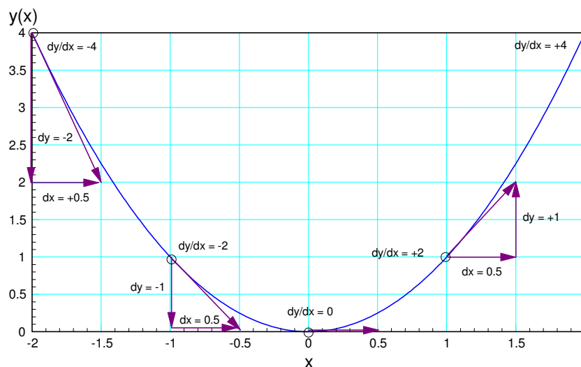
Figure 5: The derivative of a function can be found using graphical methods
