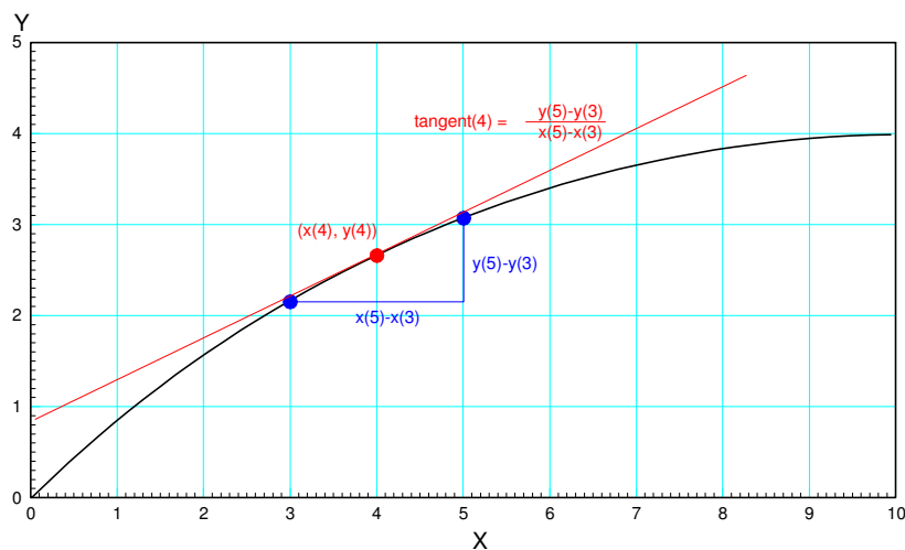
Figure 12: The derivative at x=4 can be computed as the change in y over the change in x
