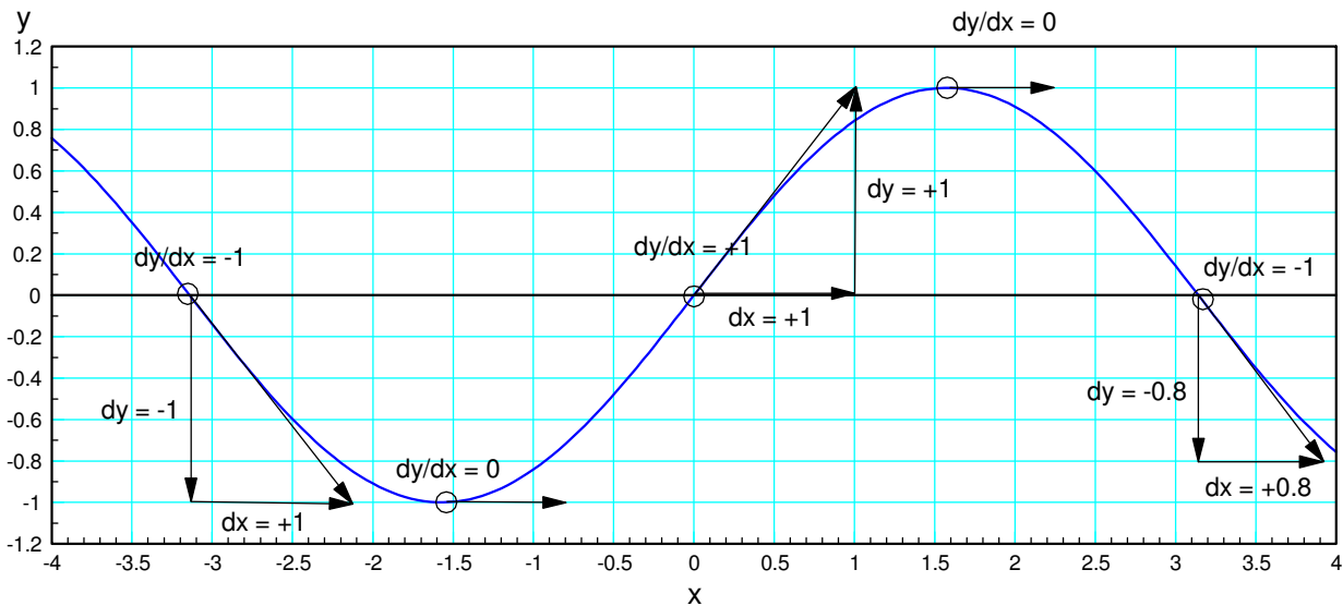
Figure 7: To find the derivative, start by computing the slope at several points
